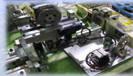
Module connector assembly jig
